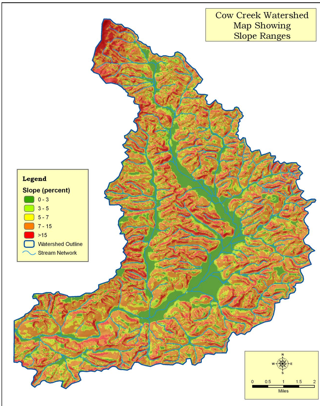
Figure 4. Slope Map
