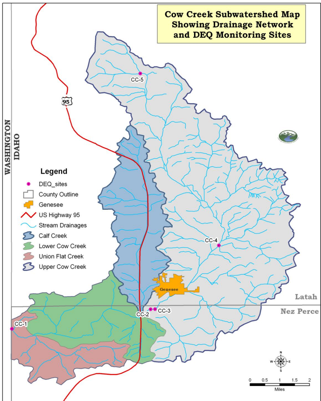
Figure 5. Subwatersheds Map
