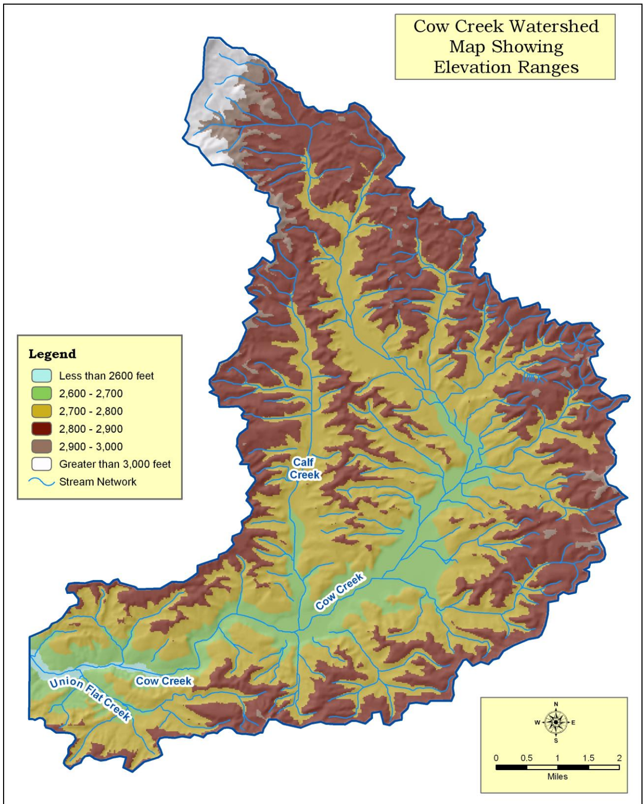
Figure 3. Elevation Map
