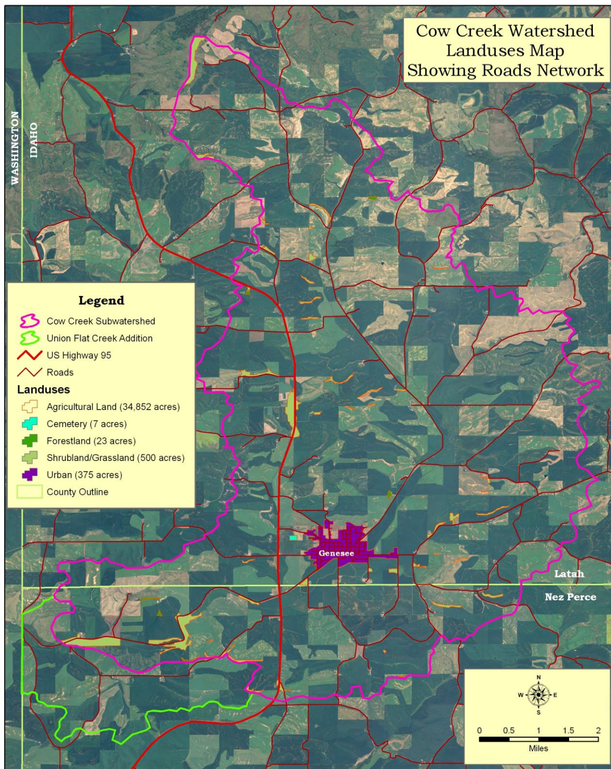
Figure 6. Landuses Map
