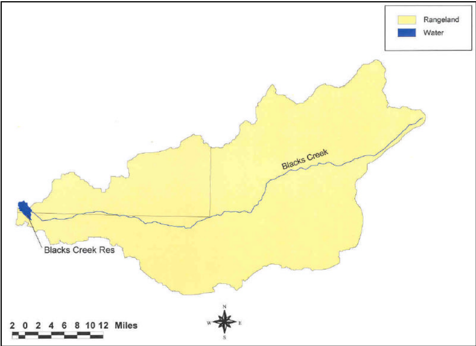
Figure 5. Blacks Creek Land Use (modified from IDWR 1994 data)
