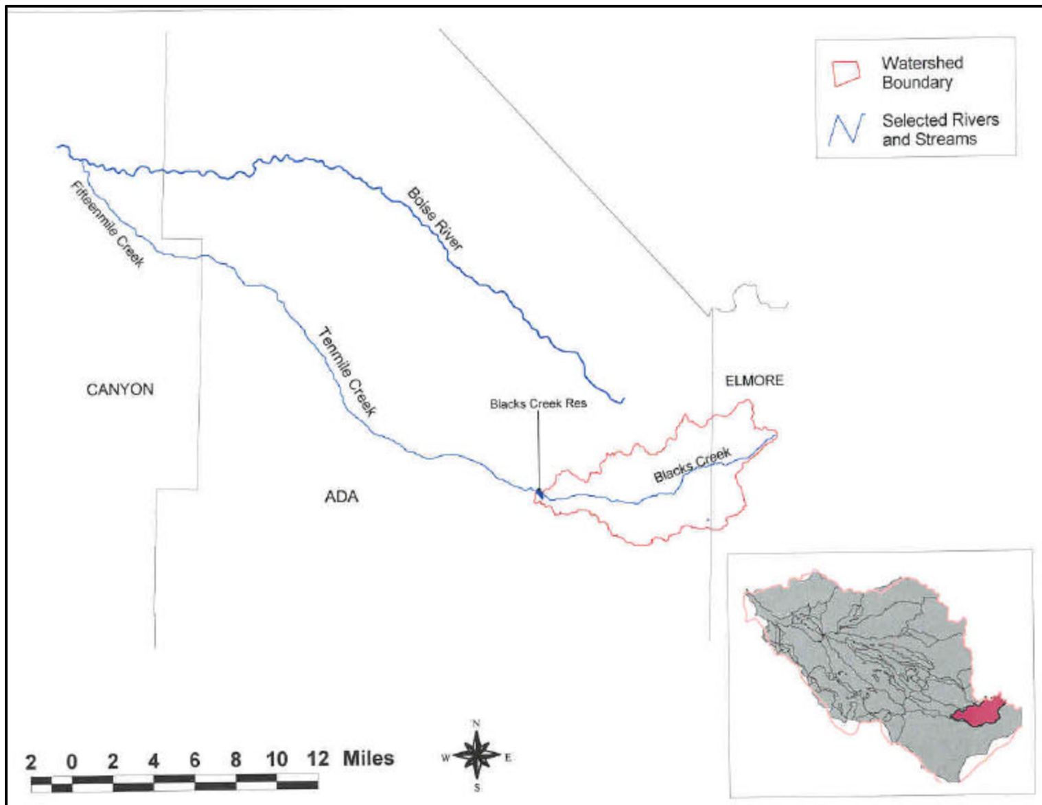
Figure 2. Blacks Creek Watershed
